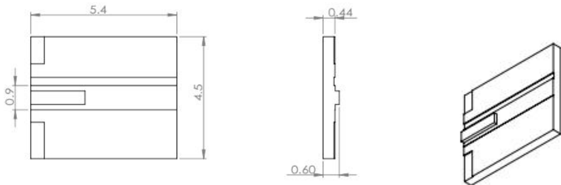
CoS Package
