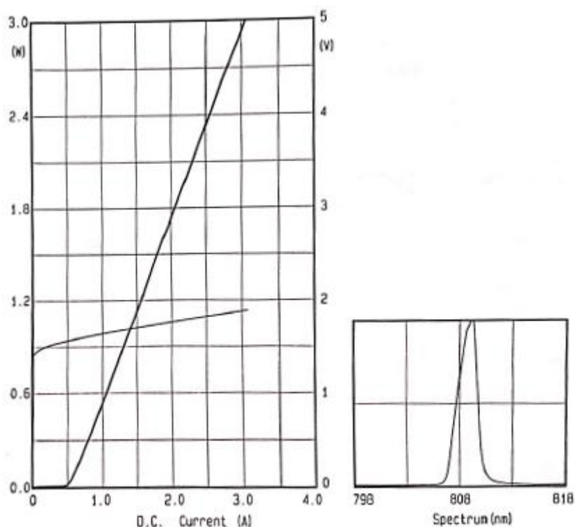
P-I-V Curve
